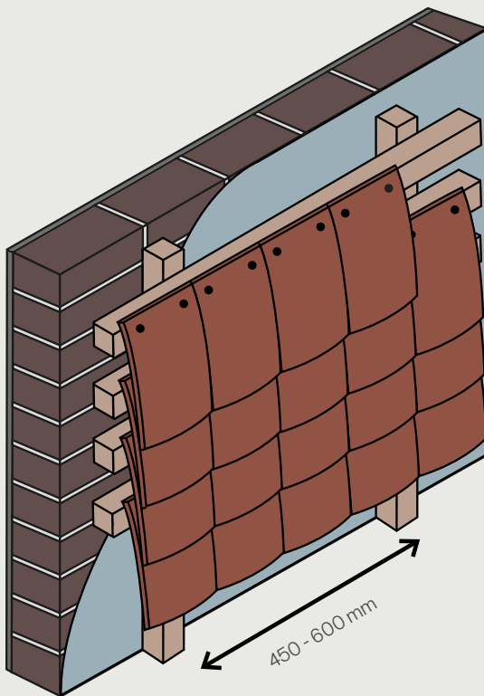
Figure 1: Typical Vertical Tiling Assembly
