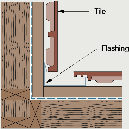
Figure 2: Internal Corner Detail
