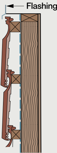
Figure 4: Vertical Tiling Sill Detail
