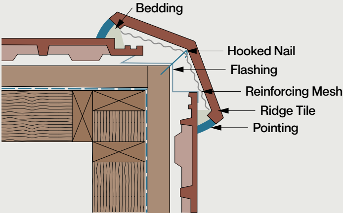
Figure 3: External Corner Detail
