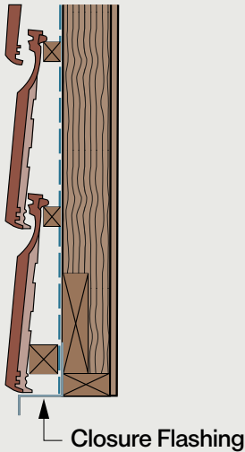
Figure 5: Vertical Tiling Above a Lintel Detail
