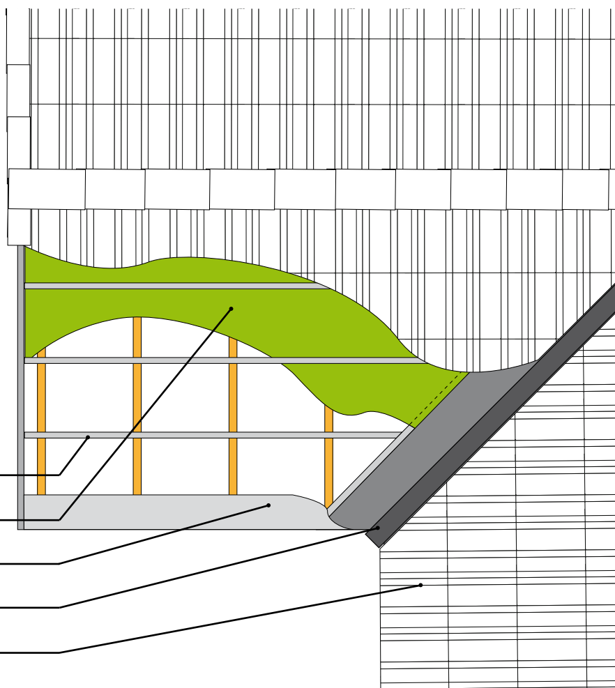
Figure 1 | BAL Roof plan view
