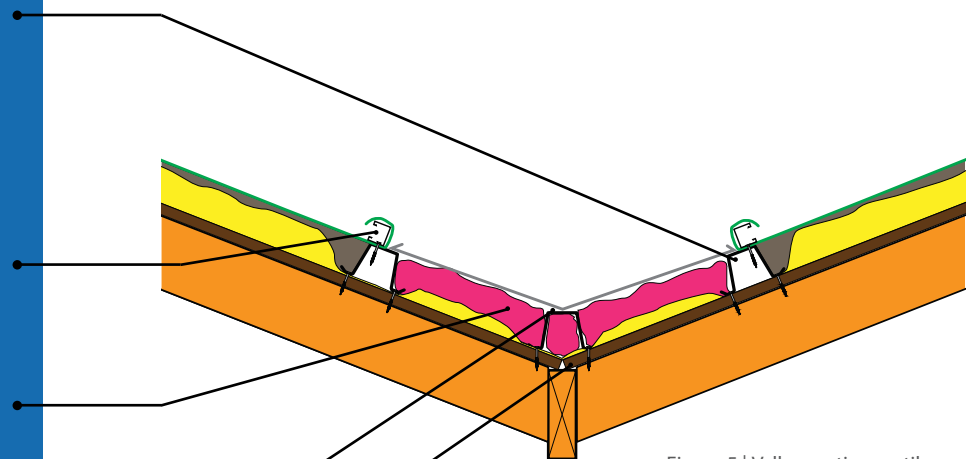
Figure 5 | Valley section no tiles
