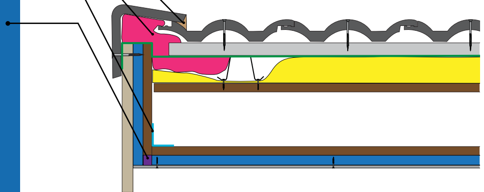
Figure 8 | Barge section (Shaped Profile)
