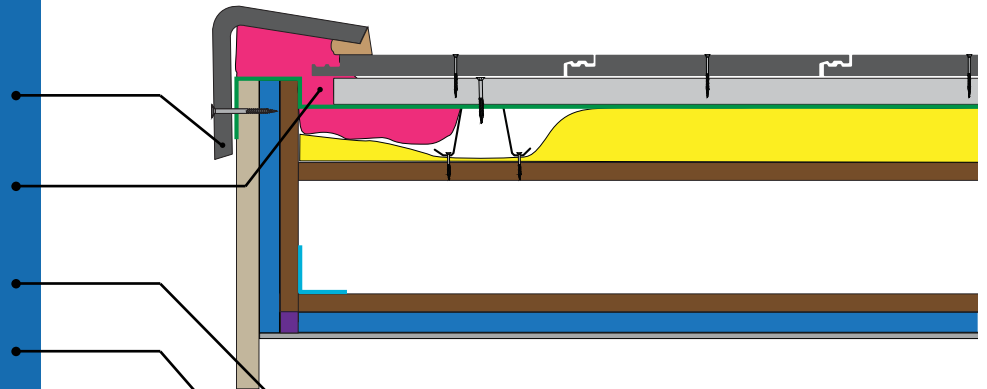
Figure 7 | Barge section (Flat Profile)
